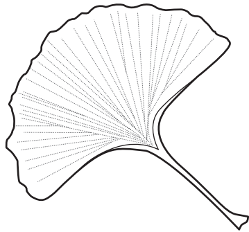
Dichotomous
