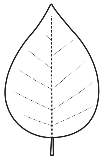
Pinnate
