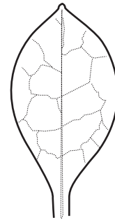
Reticulate
